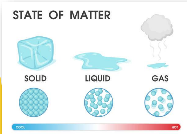
States of matter
